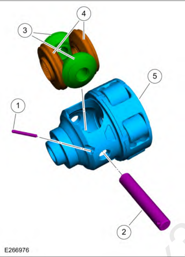
Differential Exploded View
